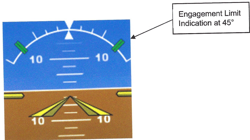
Figure 7-1: Nominal Roll Attitude ESP Engagement Limit Indications
